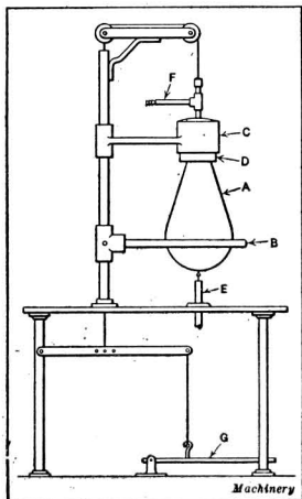
Fig. 22. Piercing Bulb
